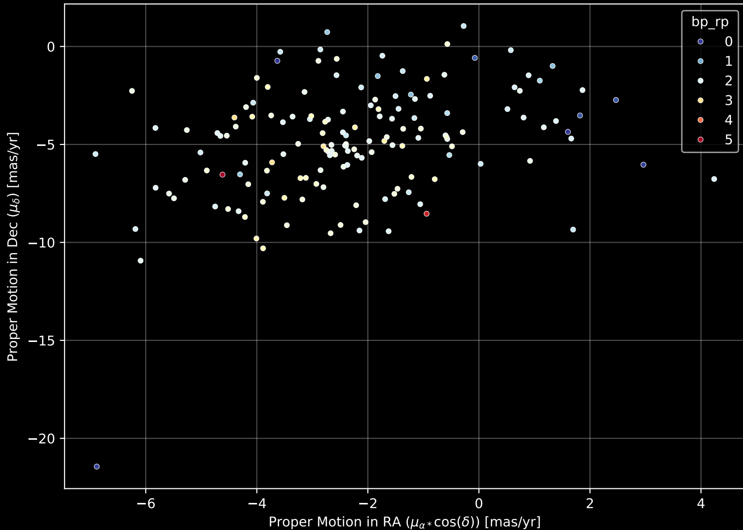
APOGEE DR17 Field: [N6441] Proper Motion Diagram (n= 153)
