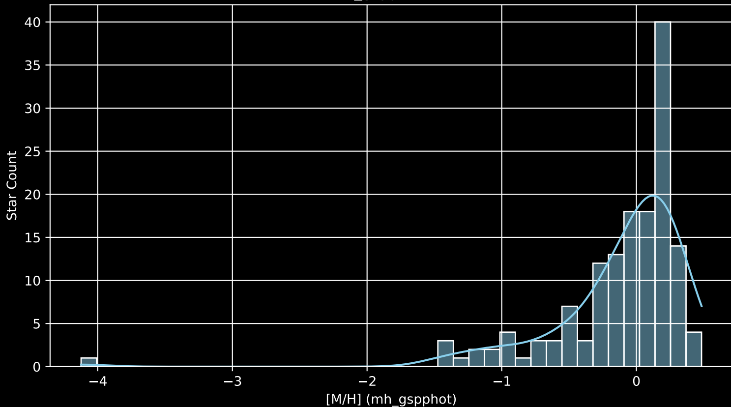
APOGEE DR17 Field: [N6441 [M/H] (mh_gspphot) (n= 149)
