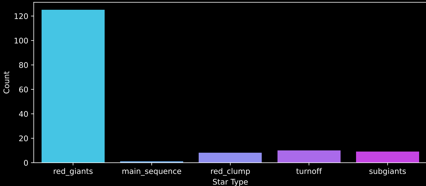
APOGEE DR17 Field: [N6441] Count plot of Star Type
