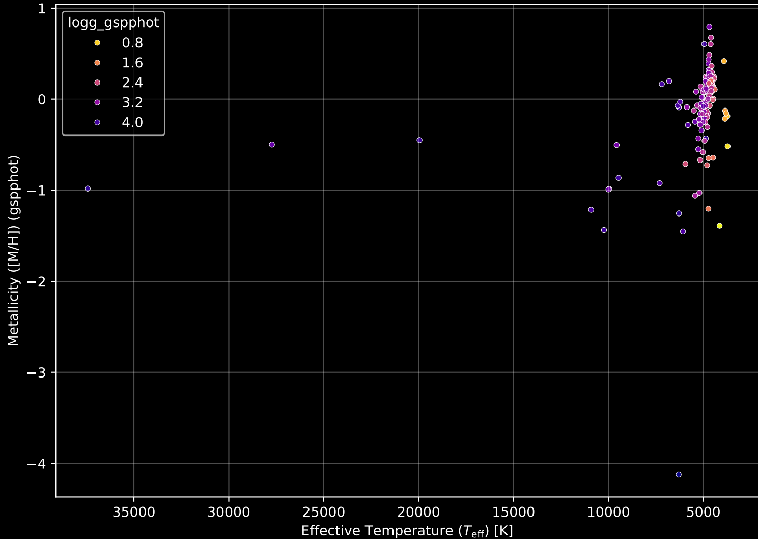
APOGEE DR17 Field: [N6441] Stellar Population Parameters (n= 153)
