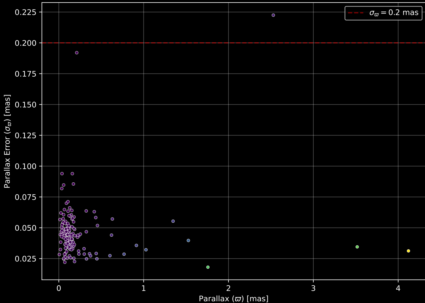
APOGEE DR17 Field: [N6441] Parallax Quality (n= 153)
