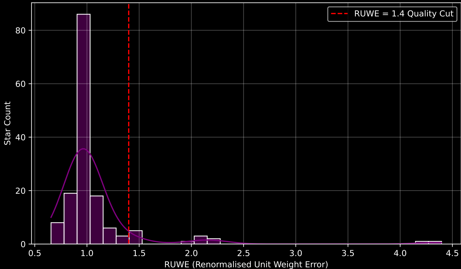
GAPOGEE DR17 Field [N6441] RUWE Distribution (n= 153)
